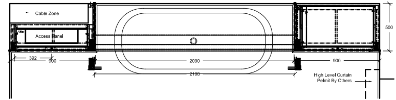
1:10 Plan Section
