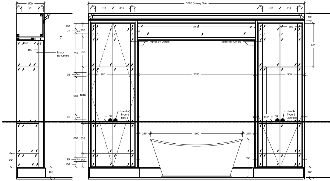
1:10 Side Elevation
