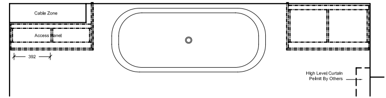
1:10 Plan Section of Plinth
