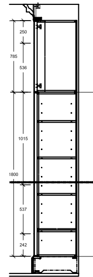
1:10 Side Section R/H Unit
