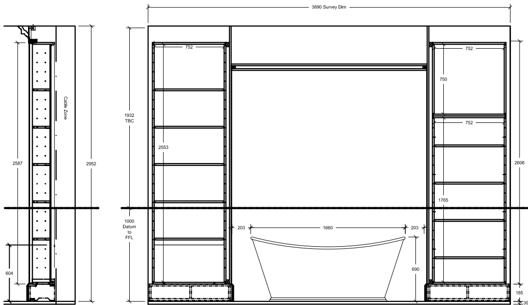
1:10 Side Section L/H Unit
