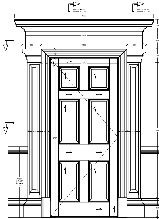
1:5 Elevation from Hall Side
