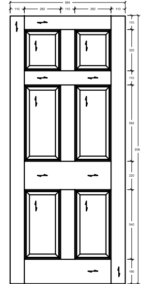
1:5 Elevation of Door (Hall Side) Light American Walnut Finish
