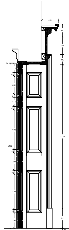
1:5 Height Section C-C
