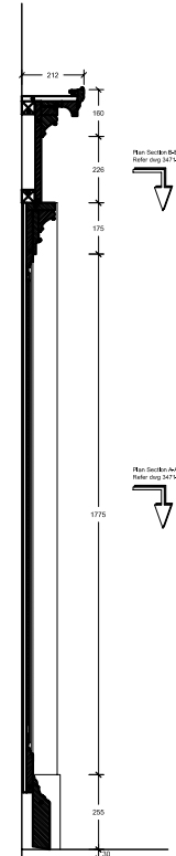
1:5 Height Section D-D
