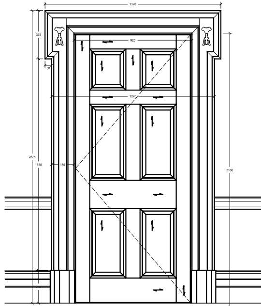
1:5 Elevation from Majlis Room Side
