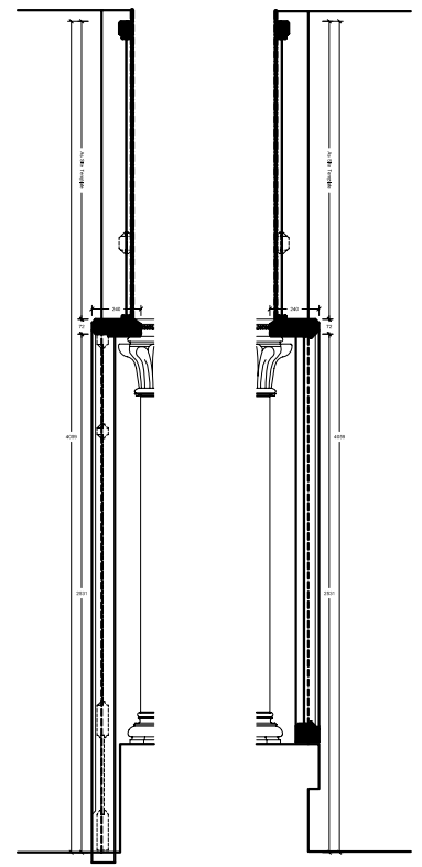
1:5 Height Section through Door Frame
