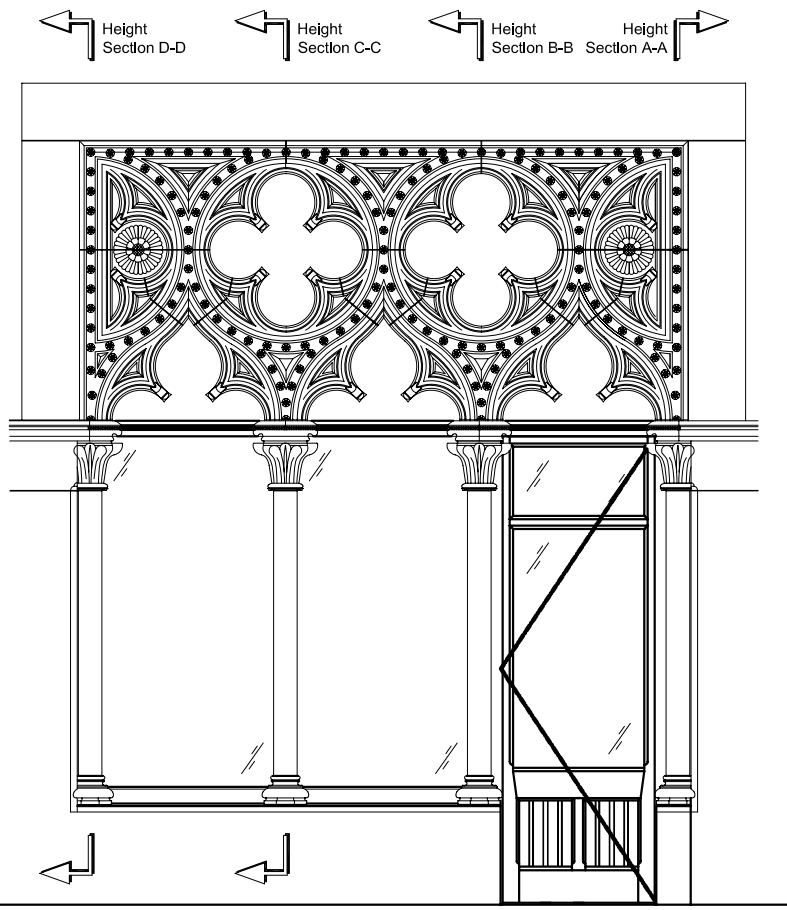
1:5 Hall Side Elevation
