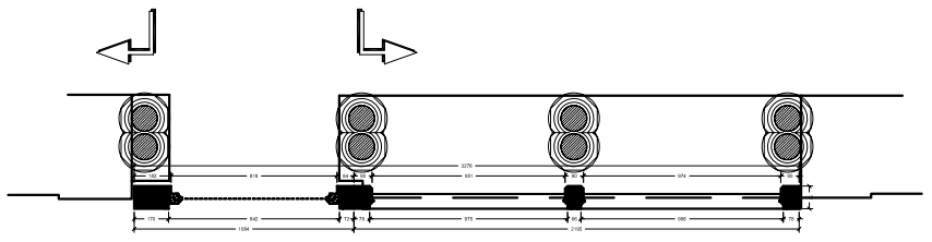
1:5 Plan through Frame & Glazing
