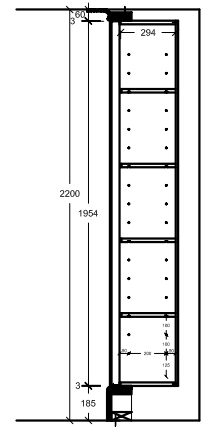
1:10 Height Section C-C
