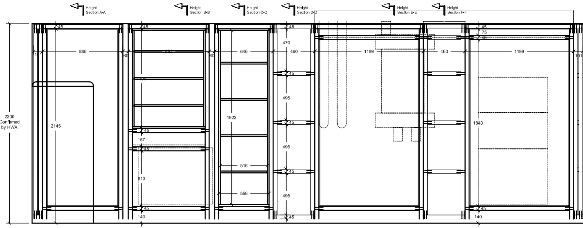
1:10 Front Height Section
