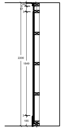
1:10 Height Section F-F
