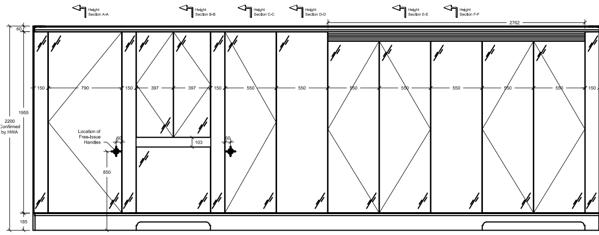
1:10 Front Elevation
