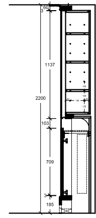
1:10 Height Section B-B
