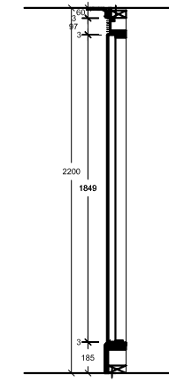
1:10 Height Section E-E
