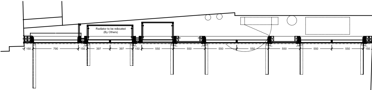
1:10 Plan Section (High Level)
