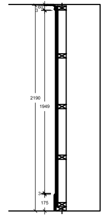
1:10 Height Section D-D
