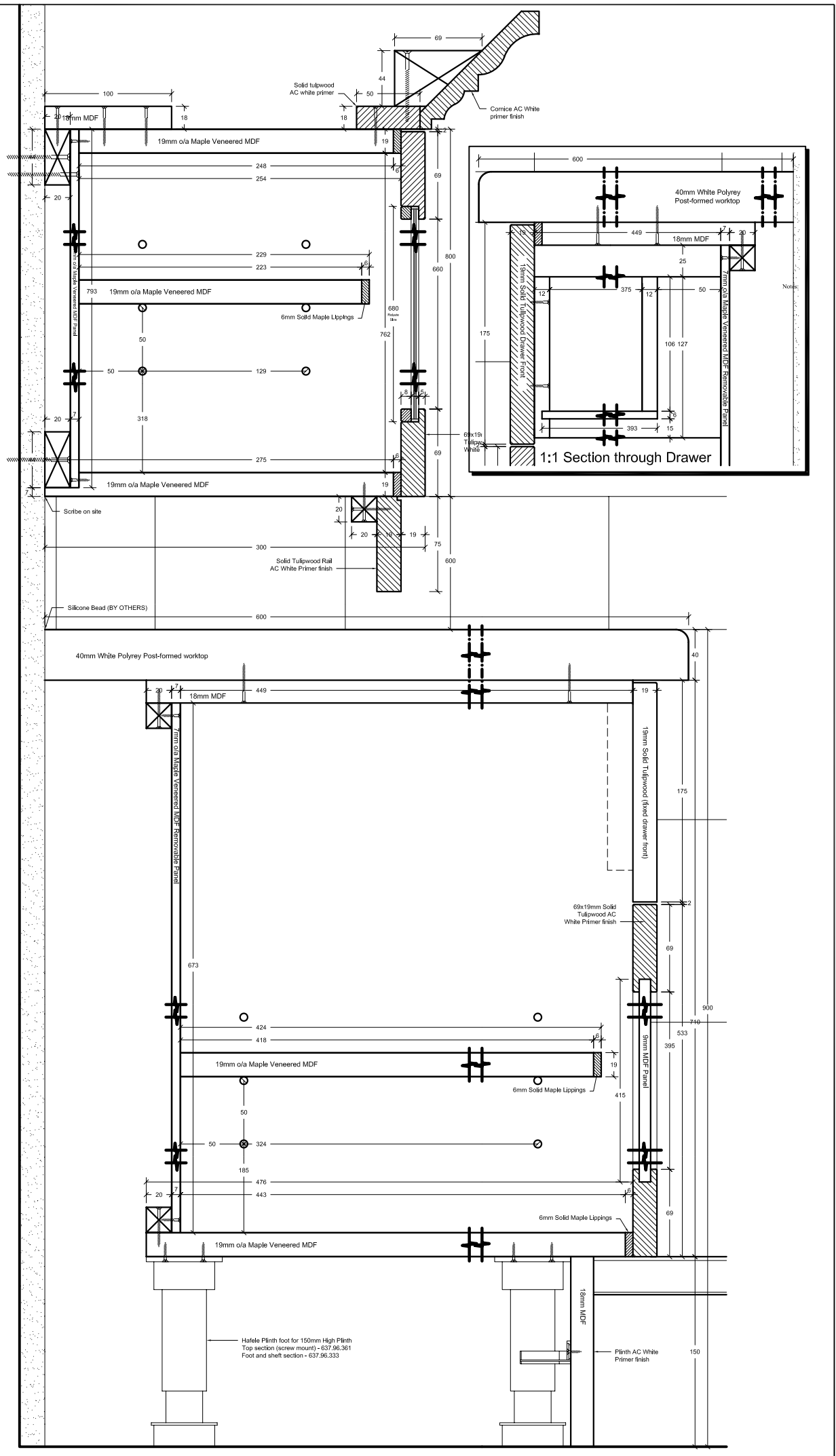
1:1 Section thru ends
