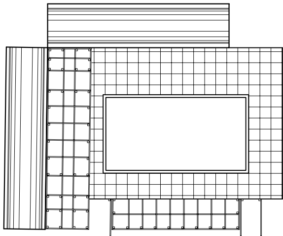
1:50 Plan of Joists/Posts
