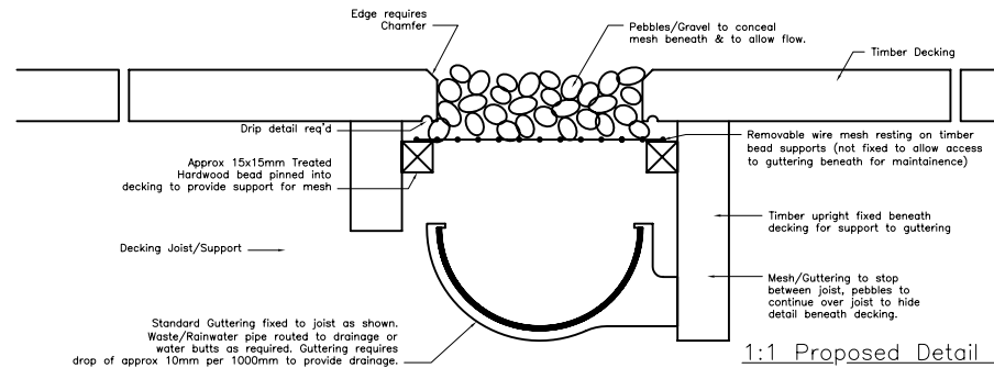
1:1 Proposed Detail for drainage (Detail & Sizes awaiting confirmation)
